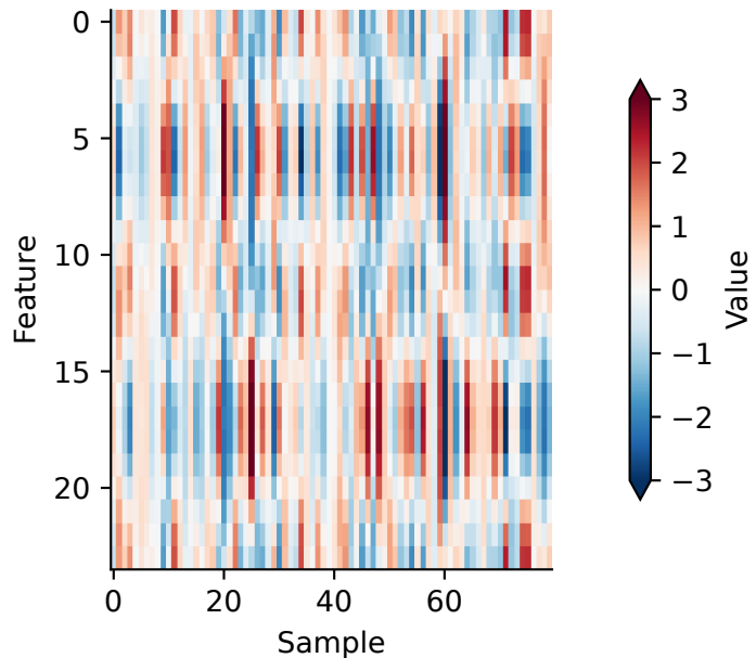
VBPCA reconstruction
